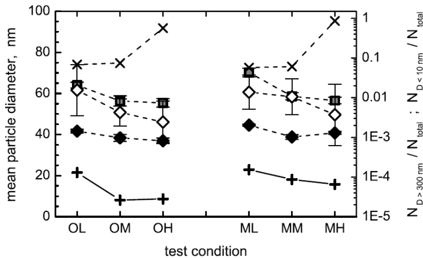
Figure 2-2 mean particle diameter and normalised number concentration (Source Petzold et al)
