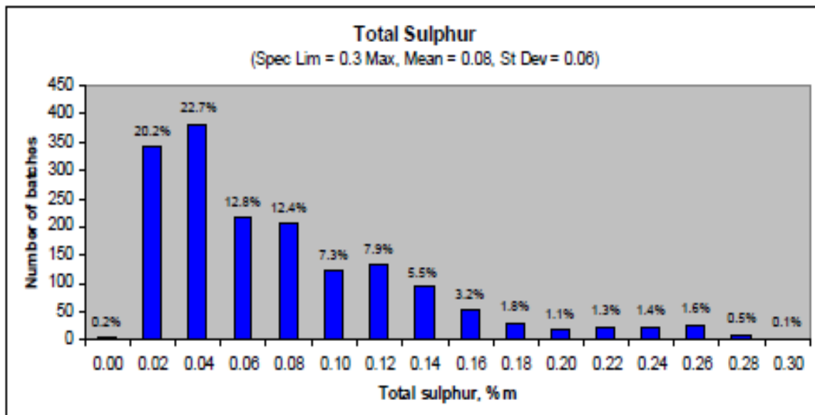
Figure 5-1: Batch to batch variation in sulphur content for UK jet fuel supplied in 2008
