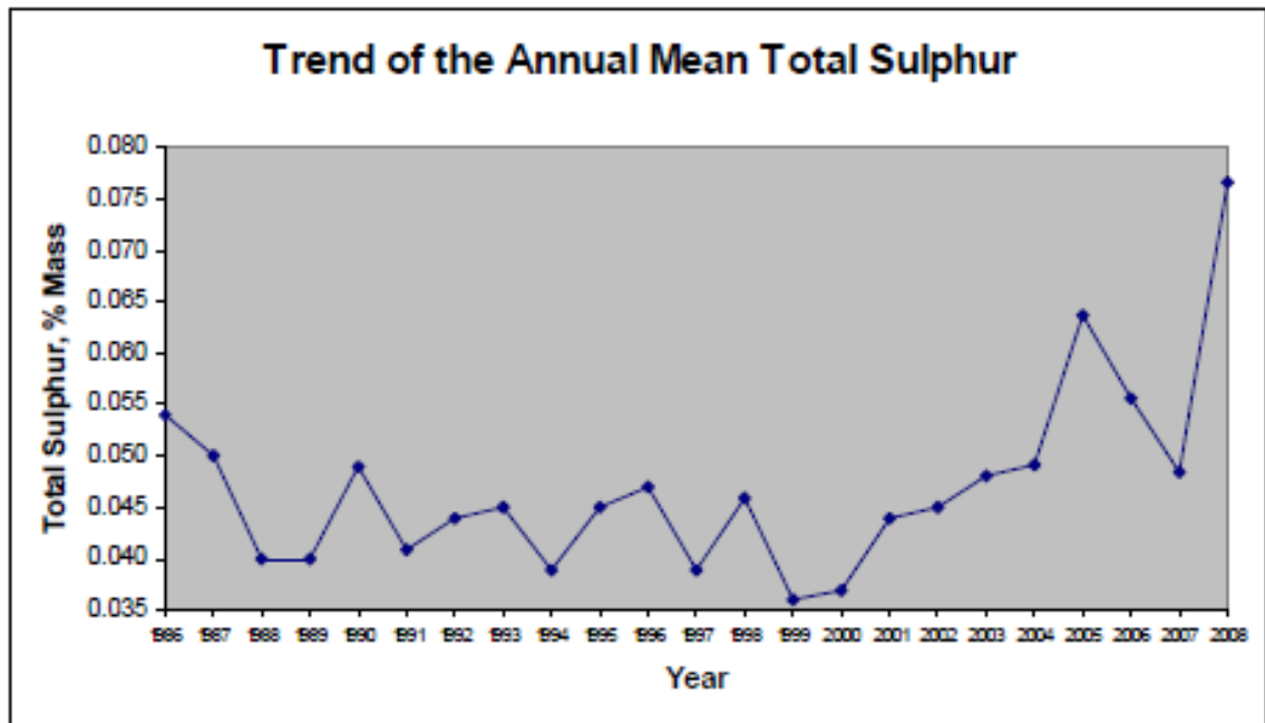
Figure 5-2: Variations in the annual mean sulphur content for UK jet fuel supplied between 1986 and 2008
