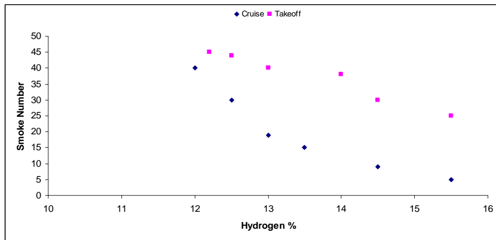
Figure 2-3 Smoke number against the hydrogen content of the fuel (reproduced from Lefebvre[14], relevant to JT8D combustor)
