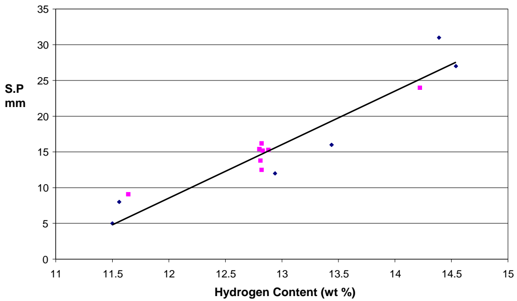
Figure 2-4 Relationship between smoke point and hydrogen content Source Moses et al and Lefebvre et al
