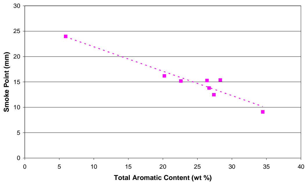
Figure 2-5 Smoke point as a function of aromatic content
