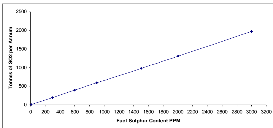
Figure 3-1 Tonnes of SO 2 produced per annum at Heathrow
