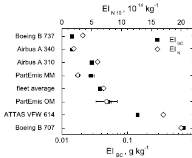
Figure 2-1 Characteristics of particulates measured from the HES and compared to those of other engines. (SOURCE Petzold and Schumann et al [9] )
