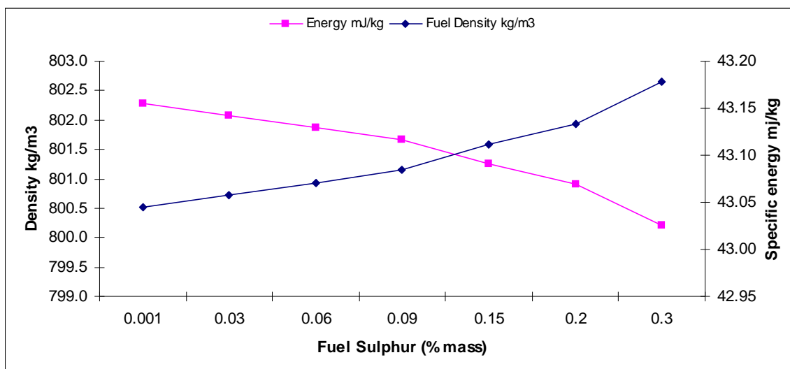
Figure 7-1 Density and specific energy versus fuel sulphur content
