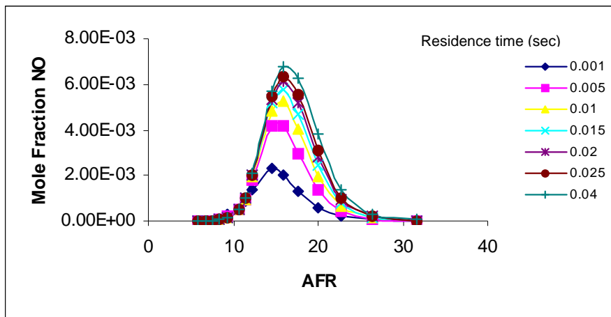
Figure 7-2 NOx production as a function of residence time and AFR
