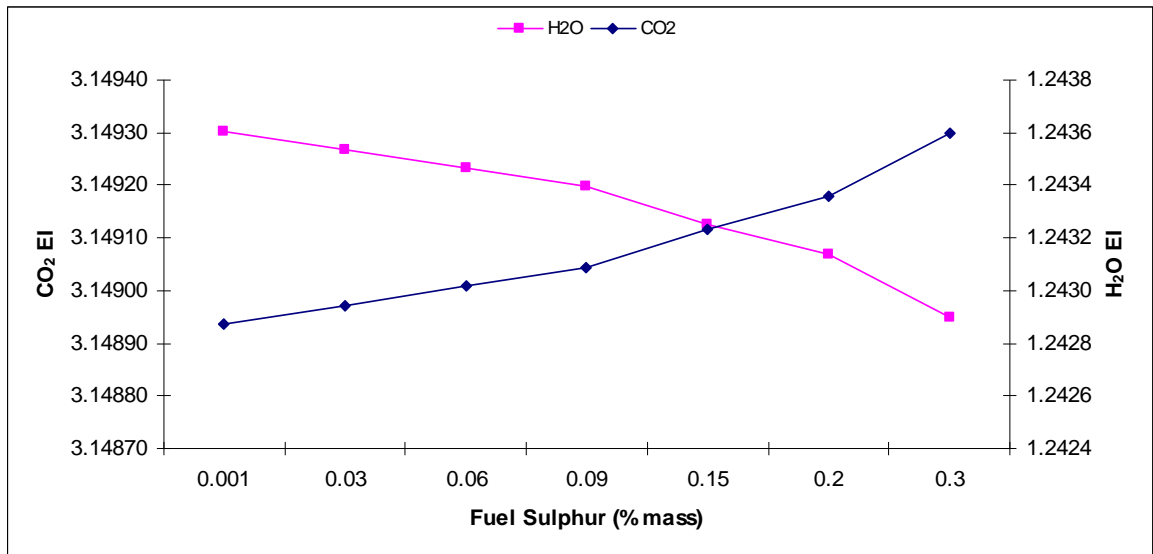
Figure 7-3 EI CO 2 and H 2 O as a function of FSC
