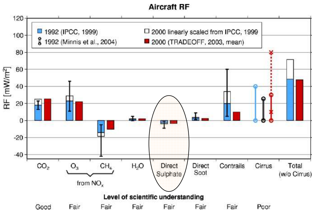
Figure 4-1 Global radiative forcing (RF) [mW/m 2 ] from aviation estimated for the years 1992 and 2000, based on IPCC (1999) and TRADEOFF results. The whiskers denote the 2/3 confidence intervals of the IPCC (1999) values. The lines with the circles at the end display different estimates for the possible range of RF from aviation induced cirrus clouds. In addition the dashed line with the crosses at the end denotes an estimate of the range for RF from aviation-induced cirrus. The total does not include the contribution from cirrus clouds. Note that there are concerns about RF as a metric for climate change; for example, some RFs (e.g., those from contrails, induced cirrus clouds, and ozone from NO x emissions) are
